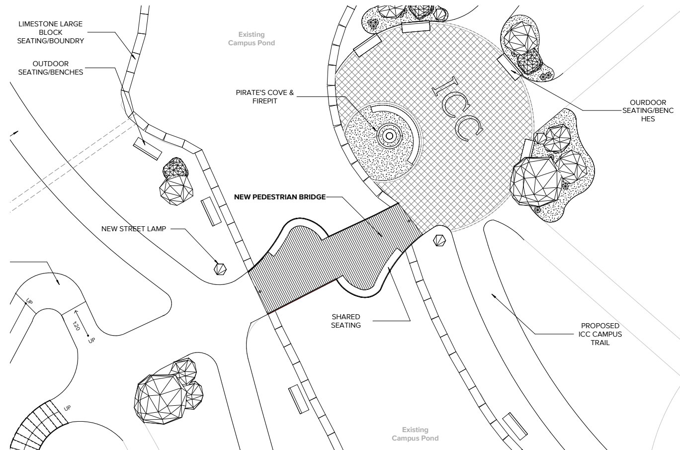
Conceptual Plan of new ICC Pedestrian Bridge
